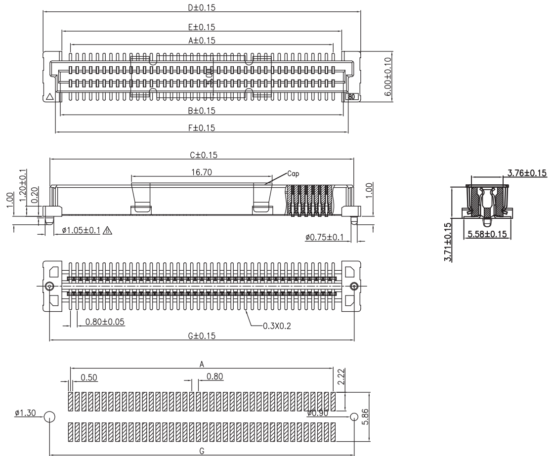
PCB LAYOUT
